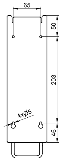
Bohrbild | drilling pattern
