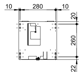
Bohrbild | drilling pattern
