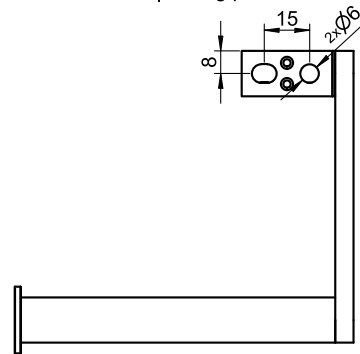
Bohrbild | drilling pattern
