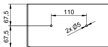
Bohrbild | drilling pattern
