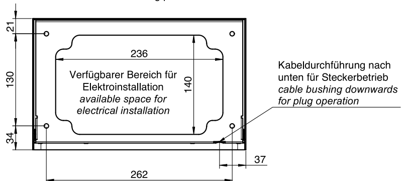
Bohrbild I drilling pattern
