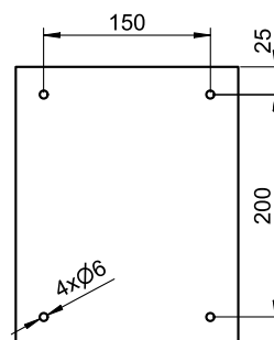
Bohrbild | drilling pattern
