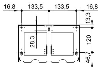
Bohrbild | drilling pattern
