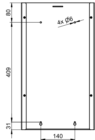
Bohrbild | drilling pattern
