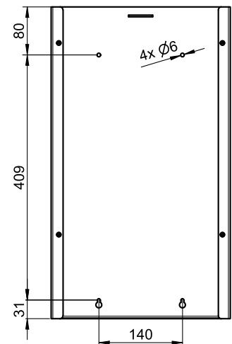
Bohrbild | drilling pattern
