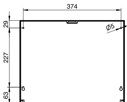
Bohrbild | drilling pattern
