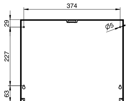
Bohrbild | drilling pattern
