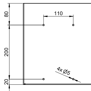
Bohrbild | drilling pattern
