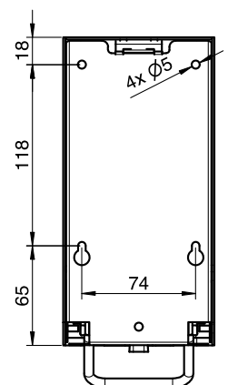
Bohrbild | drilling pattern
