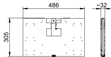
geschlossen | closed
