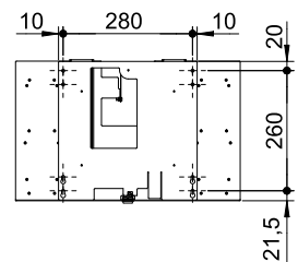
Bohrbild | drilling pattern
