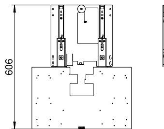
offen | open
