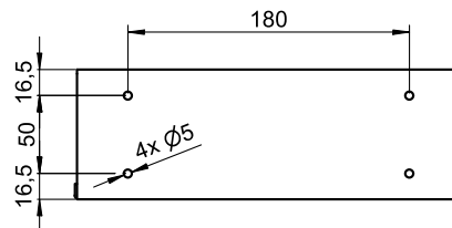
Bohrbild | drilling pattern
