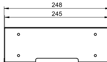
Bohrbild | drilling pattern
