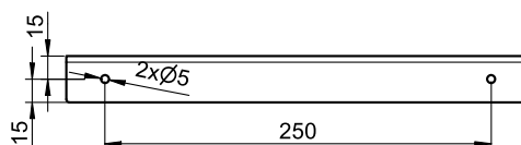
Bohrbild | drilling pattern
