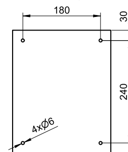
Bohrbild | drilling pattern
