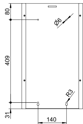
Bohrbild | drilling pattern
