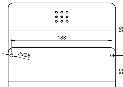
Bohrbild | drilling pattern
