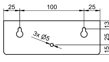
Bohrbild | drilling pattern
