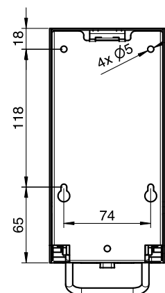
Bohrbild | drilling pattern
