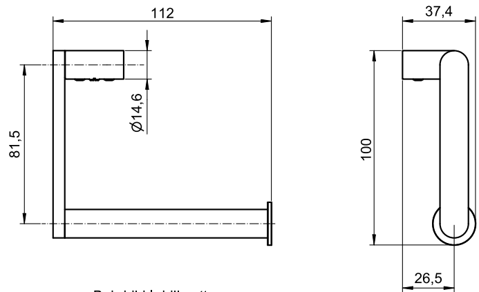
Bohrbild | drill pattern
